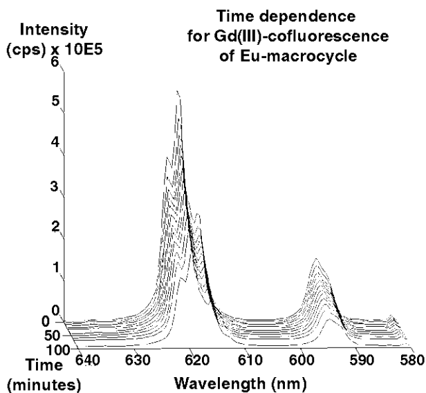
Figure 6. Time-dependence plot for the emission intensity of the [\text{Eu}(\text{macrocycle})(\text{acetate})_2](\text{acetate}) complex in a Gd-containing optimized cofluorescence solution. Only one band arising from the {}^5\text{D}_0 \rightarrow {}^7\text{F}_0 transition of the Eu-macrocycle transition occurs at ca. 580 nm, showing that only one emitting species is present. Furthermore, the peak pattern of the band corresponding to the {}^5\text{D}_0 \rightarrow {}^7\text{F}_2 transition is constant in time, even though the intensity decreases, showing that the chemical nature of the emitting species remains unchanged.
