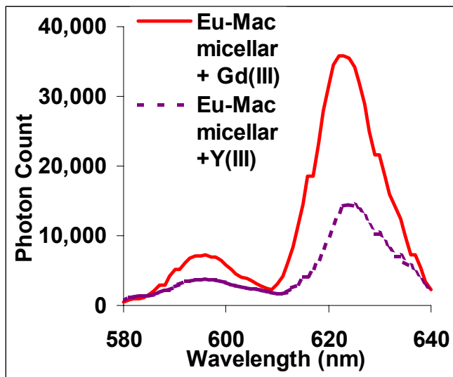
Figure 4. Emission spectra (Excitation: 375 nm) of [Eu-Macrocycle(acetate) 2 ](acetate) in two cofluorescence solutions, one containing Gd(III) and the other containing Y(III) as the donor. (All other reagents are present at the same concentrations, see Table 1). The Gd(III) provides significantly stronger, 2.6 fold, enhancement relative to Y(III).
