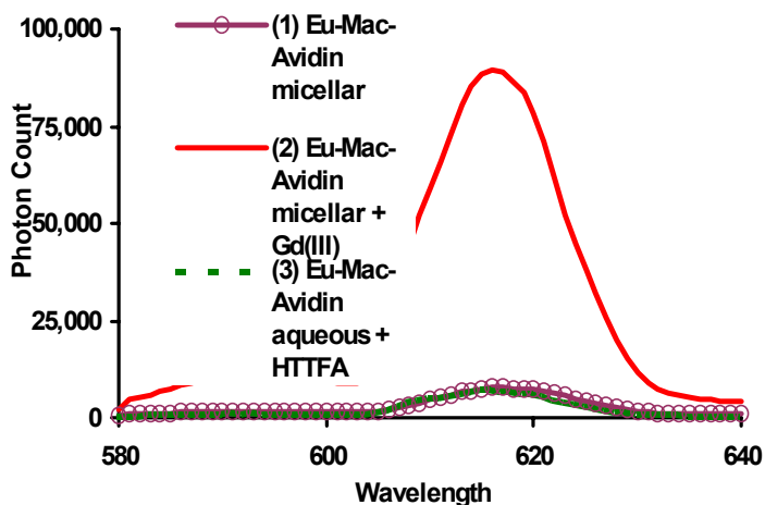
Figure 5. Emission spectra (Excitation: 365 nm) of the Eu-Mac-Avidin at a concentration of 2.2 \times 10^{-6} mol Eu(III)/L in: (1) A cofluorescence-optimized aqueous micellar solution. (2) Identical to the preceding solution but with Gd(III) chloride ( 1.2 \times 10^{-4} M). (3) An aqueous buffered solution with only HTTFA added.
