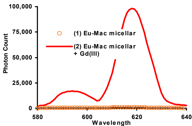
Figure 2. Emission spectra (Excitation: 375 nm) of: (1) A solution of [\text{Eu-Macrocycle}(\text{acetate})_2](\text{acetate}) ( 2.28 \times 10^{-7} M) in the optimized-cofluorescence matrix without Gd(III). (2) An identical solution but with Gd(III) chloride ( 1.2 \times 10^{-4} M). In (2), the integrated emission intensity between 613 and 623 nm is increased over 100-fold by the addition of the Gd(III).
