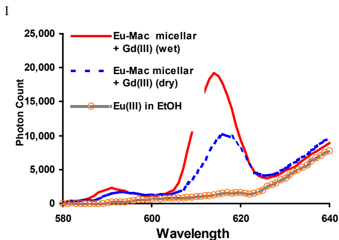
Figure 7. Reflectance emission spectra (Excitation: 375 nm) of wet and dry spots obtained from a cofluorescence-optimized aqueous micellar solution of [\text{Eu-Mac}(\text{acetate})_2](\text{acetate}) ( 2.3 \times 10^{-7} M), and of a wet spot from an ethanol solution of \text{Eu}(\text{III}) ( 2.3 \times 10^{-7} M) with only HTTFA added. Spectra were recorded under identical instrumental settings and the background from the paper was subtracted; however, the reflectance behavior of the paper changes upon drying. The rise in the curve above 630 nm is due to scattering from the paper.
